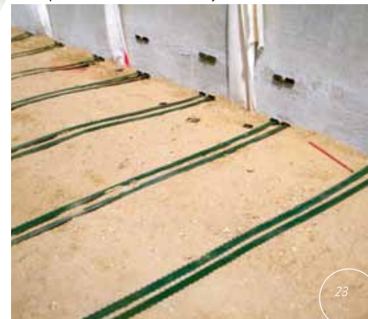
EcoStrap™ HA® reinforcements in Chessy.
